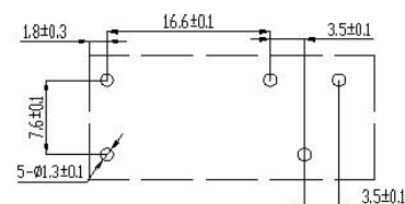
BOTTOM VIEW (1C)
