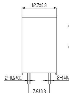
BOTTOM VIEW (1B)
